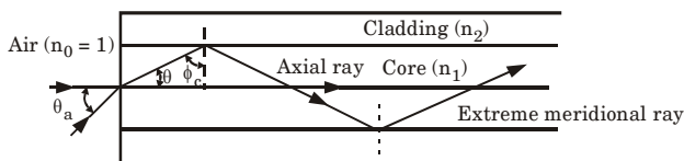
Fig. 2.13.1. The paths taken by the axial and an extreme meridional ray in a perfect multimode step index fiber.
