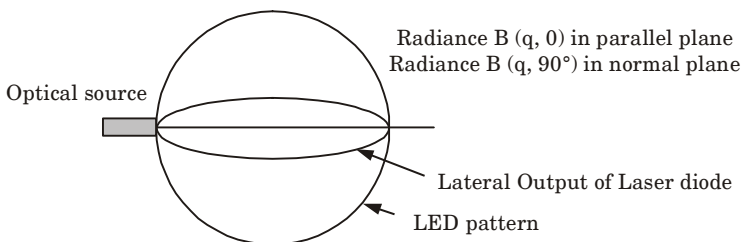
Fig. 4.1.2. Radiance pattern of Lambertian source.
