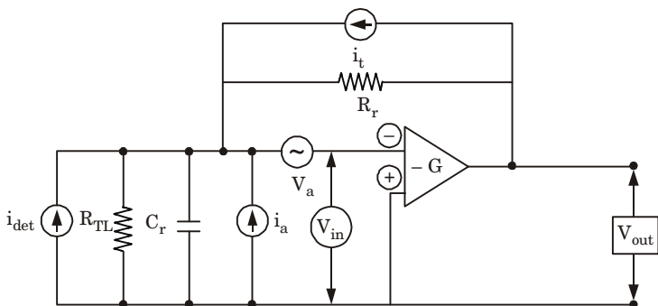
Fig. 4.22.3. An equivalent circuit for the optical fiber receiver incorporating a transimpedance (current mode) preamplifier.
