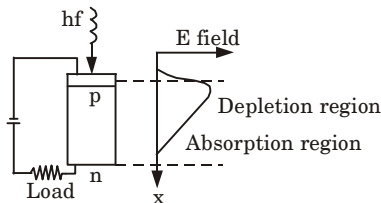
Fig. 4.9.1. p-i-n photodiode showing combined absorption and depletion region.
