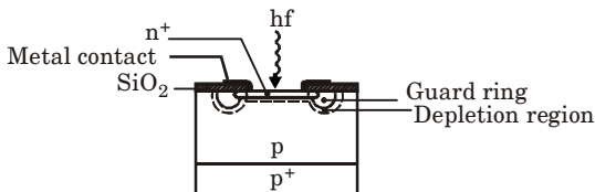
Fig. 3. Structure of a silicon avalanche photodiode with guard ring.
