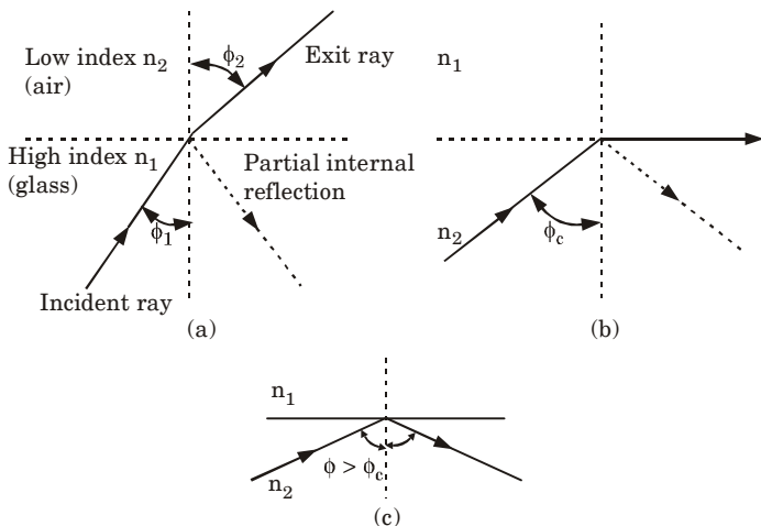
Fig. 8. Light rays incident on high to low refractive index interface ( e.g. glass-air): (a) refraction; (b) the limiting case of refraction showing the critical ray at an angle \phi_c ; (c) total internal reflection where \phi > \phi_c .
