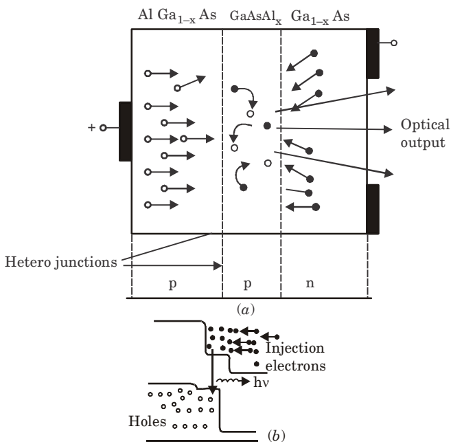
Fig. 7. (a) The double heterojunction LED, layer structure. (b) The corresponding energy band diagram.
