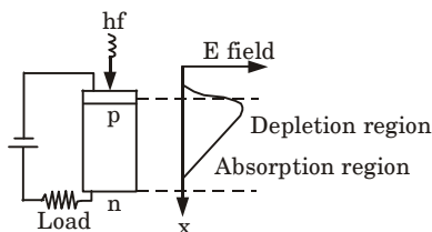
Fig. 3. p - i - n photodiode showing combined absorption and depletion region.
