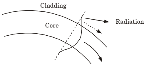
Fig. 11. An illustration of the radiation loss at a fiber bend.
