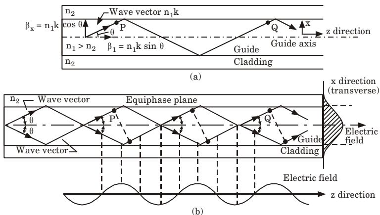
Fig. 4. The formation of a mode in a planar dielectric guide.
