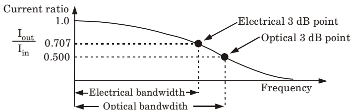
Fig. 6. The frequency response for an optical fiber system showing the electrical and optical bandwidths.
