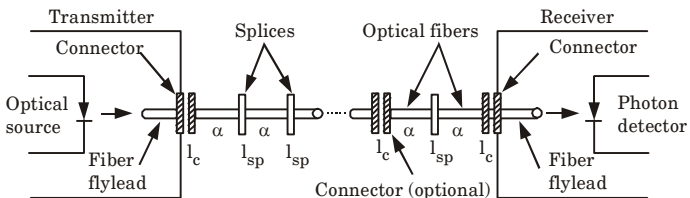
Fig. 5.11.1. Optical power loss model for a point-to-point link.
