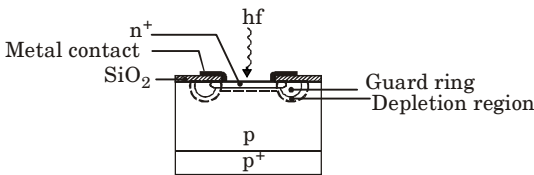
Fig. 4.12.2. Structure of a silicon avalanche photodiode with guard ring.
