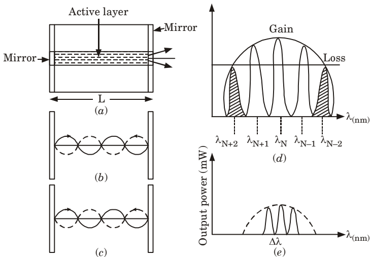
Fig. 3.14.1. Fabry-Perot Laser diode; (a) A Laser diode; (b) Fabry-Perot resonator with arbitrary wave; (c) Fabry-Perot resonator with standing wave; (d) Gain loss Curve and possible longitudinal modes; (e) Actual multimode radiation.
