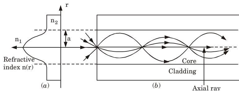
Fig. 2.14.1. A multimode graded index fiber :
