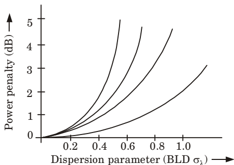
Fig. 5.13.4. Chirp induced power penalty.
