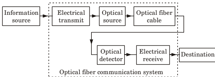
Fig. 12. The optical fiber communication system.
