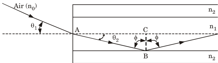
Fig. 1.6.2. The ray path for a meridional ray launched into an optical fiber in air at an input angle less than the acceptance angle for the fiber.
