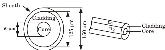
Fig. 1.4.1. Cross sectional view of an optical fiber.
