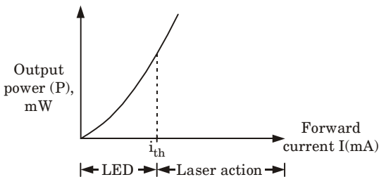
Fig. 3.10.3. Emission characteristics.
