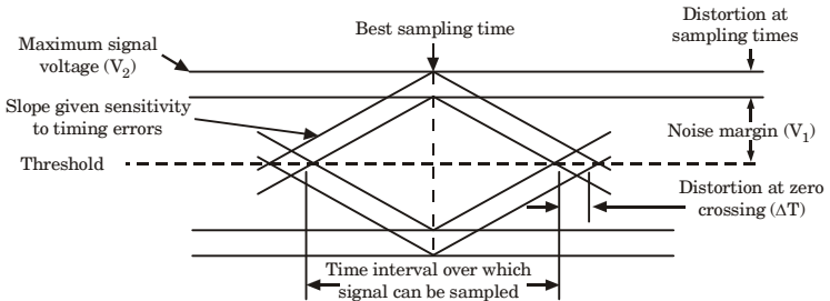
Fig. 5.6.1. Simplified eye diagram showing the key performance parameters.
