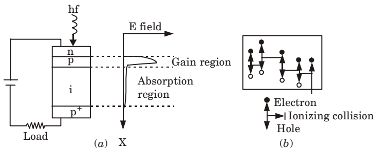
Fig. 4.12.1. (a) Avalanche photodiode showing high electric field (gain) region. (b) Carrier pair multiplication in the gain region.
