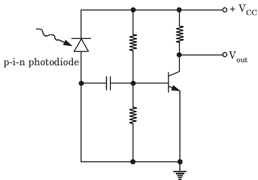
Fig. 8. A p-i-n photodiode with a grounded emitter, low input impedance voltage preamplifier.
