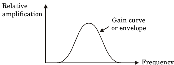
Fig. 3. The relative amplification in the Laser amplifying medium showing the broadened Laser transition line or gain curve.
