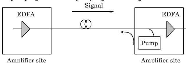
Fig. 8. Distributed Raman amplifier.
