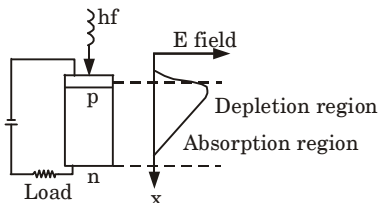
Fig. 22. p-i-n photodiode showing combined absorption and depletion region.
