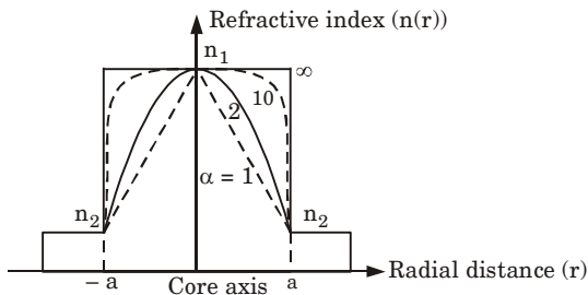
Fig. 6. Possible fiber refractive index profiles for different values of \alpha .
