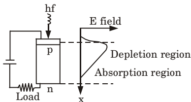
Fig. 5. p - i - n photodiode showing combined absorption and depletion region.
