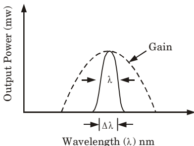
Fig. 3.15.2. Actual single mode radiation of DFB Laser diode.
