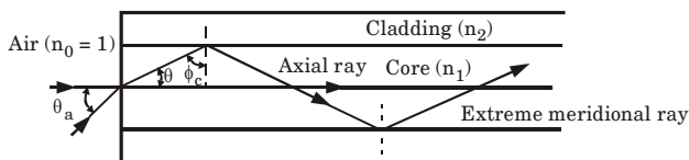
Fig. 3. The paths taken by the axial and an extreme meridional ray in a perfect multimode step index fiber.
