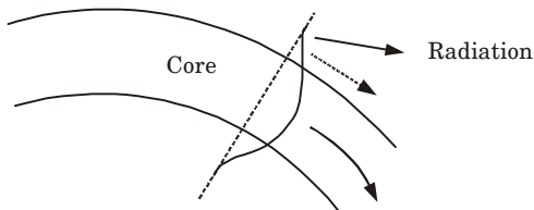
Fig. 1. An illustration of the radiation loss at a fiber bend.
