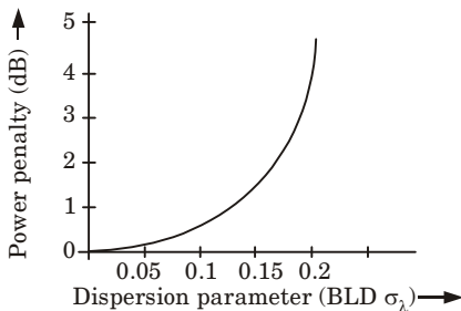
Fig. 5.13.2. Dispersion-induced power penalty.
