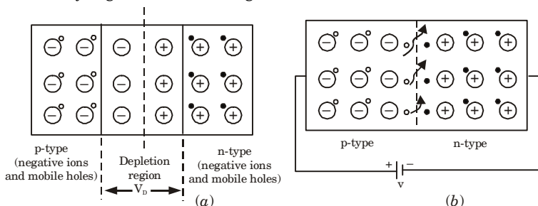
Fig. 18. Light radiation by the p - n junction of a semiconductor (a) Depletion region and Depletion voltage V_D ; (b) Light radiation as the result of electron-hole recombinations.
