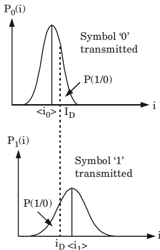
Fig. 5.3.1. Probability distributions of the photocurrent for the two transmitted symbols and selection of the decision thresholds.
