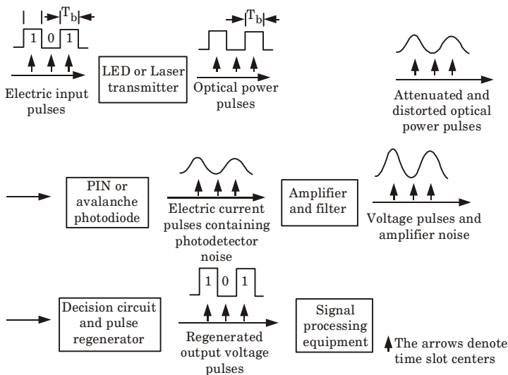
Fig. 4.23.1. Signal path through an optical data link.
