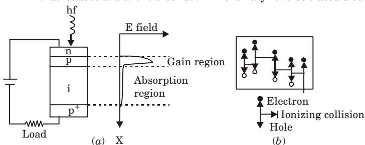
Fig. 2. (a) Avalanche photodiode showing high electric field (gain) region. (b) Carrier pair multiplication in the gain region.
