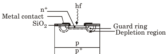
Fig. 15. Structure of a silicon avalanche photodiode with guard ring.
