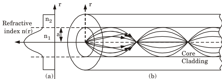
Fig. 1.21.2. The refractive index profile and ray transmission in a multimode graded index fiber.
