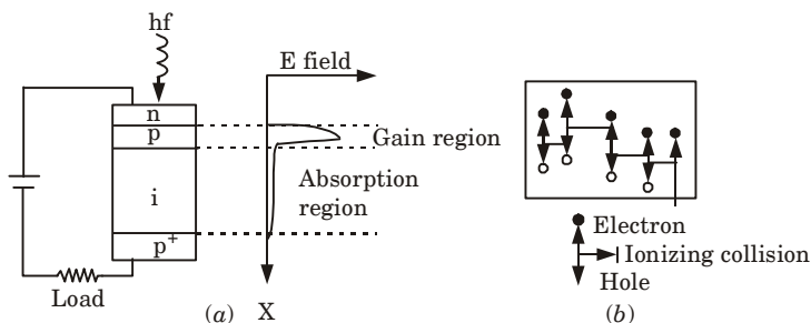
Fig. 14. (a) Avalanche photodiode showing high electric field (gain) region. (b) Carrier pair multiplication in the gain region.
