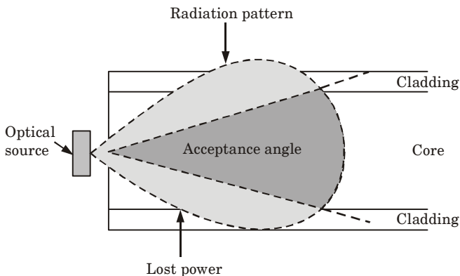
Fig. 4.2.1. Optical source coupled to fiber.
