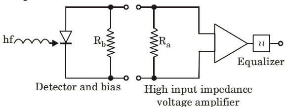
Fig. 4.22.2. High impedance integrating front end optical fiber receiver with equalized voltage amplifier.
