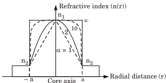
Fig. 1.21.1. Possible fiber refractive index profiles for different values of \alpha .
