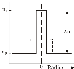
Fig. 2.18.1. Refractive index profile of a step index dispersion shifted fiber (solid) with a conventional non-shifted profile design (dashed).
