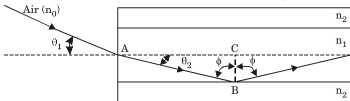
Fig. 2. The ray path for a meridional ray launched into an optical fiber in air at an input angle less than the acceptance angle for the fiber.
