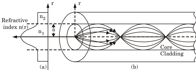
Fig. 7. The refractive index profile and ray transmission in a multimode graded index fiber.
