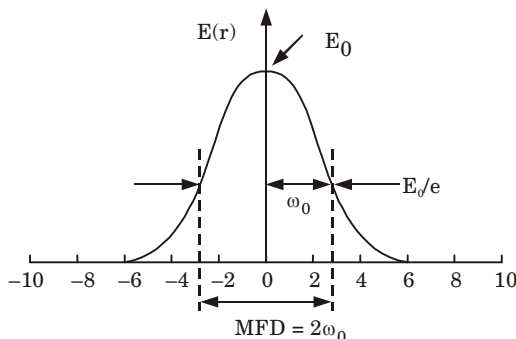
Fig. 1.24.1. Field amplitude distribution E(r) of the fundamental mode in single mode fiber illustrating the mode-field diameter (MFD) and spot size ( \omega_0 ).
