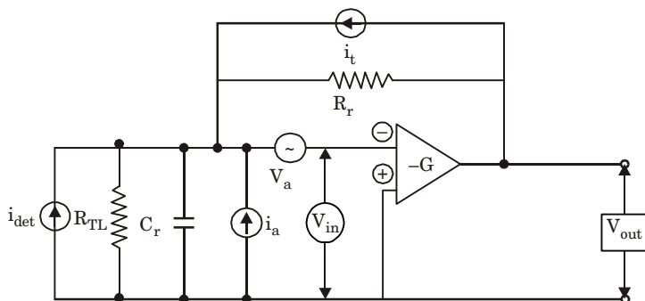
Fig. 4. An equivalent circuit for the optical fiber receiver incorporating a transimpedance (current mode) preamplifier.
