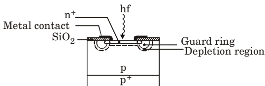
Fig. 11. Structure of a silicon avalanche photodiode with guard ring.
