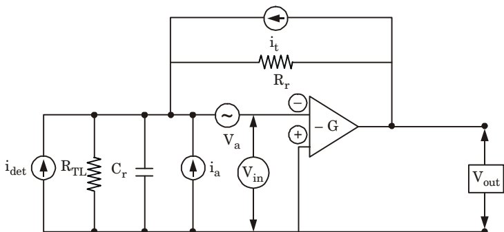
Fig. 17. An equivalent circuit for the optical fiber receiver incorporating a transimpedance (current mode) preamplifier.
