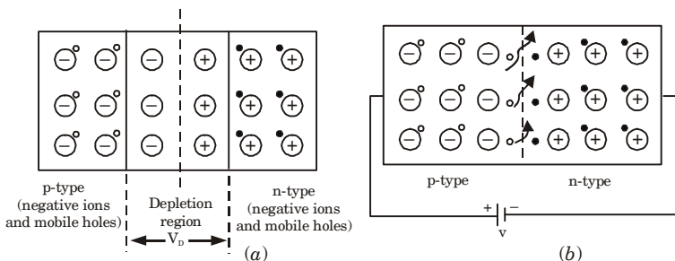
Fig. 13. Light radiation by the p - n junction of a semiconductor (a) Depletion region and Depletion voltage V_D ; (b) Light radiation as the result of electron-hole recombinations.
