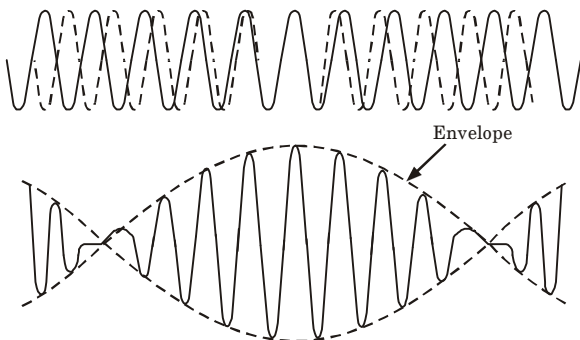
Fig. 14. Combination of two waves with nearly equal frequencies.
