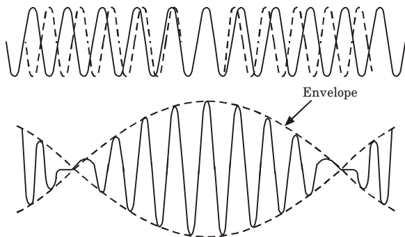
Fig. 1.14.1. Combination of two waves with nearly equal frequencies. The envelope travels at a group velocity v_g .
