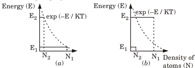
Fig. 3.13.1. Population in two energy level system : (a) Boltzmann distribution for a system in thermal equilibrium ; (b) a non-equilibrium distribution showing population inversion.
