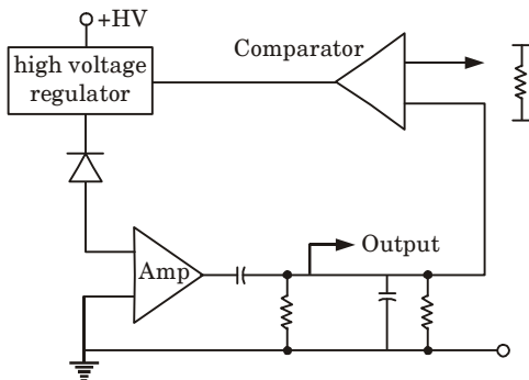
Fig. 4.14.3. Bias of an APD by peak detection and feedback to provide AGC.
