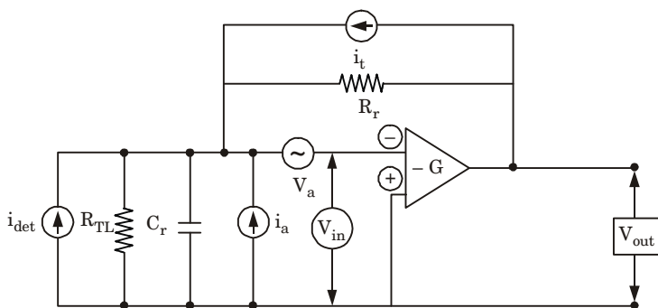
Fig. 14. An equivalent circuit for the optical fiber receiver incorporating a transimpedance (current mode) preamplifier.
