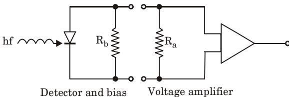
Fig. 4.22.1. Low impedance front end optical fiber receiver with voltage amplifier.
