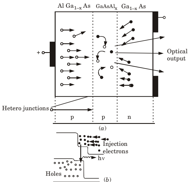
Fig. 3.3.1. (a) The double heterojunction LED, layer structure. (b) The corresponding energy band diagram.
