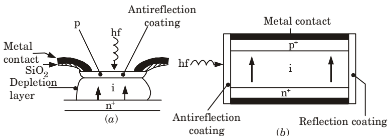
Fig. 5. p - i - n photodiode showing combined absorption and depletion region.
