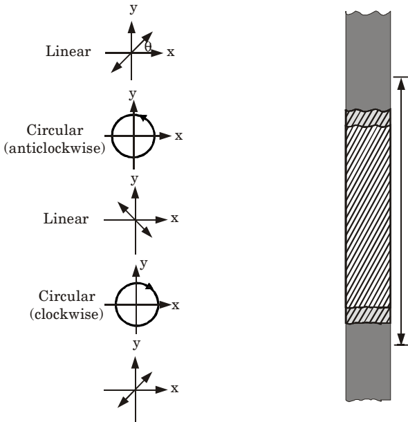
Fig. 16. An illustration of the beat length in a single mode optical fibre. where \beta_x and \beta_y are propagation constants for two modes along x and y direction.
