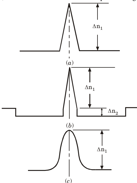
Fig. 6. Refractive index profiles for graded index dispersion shifted fibers; (a) triangular profile; (b) depressed-cladding triangular profile, (c) Gaussian profile.
