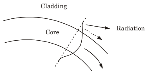
Fig. 2.5.1. An illustration of the radiation loss at a fiber bend.
