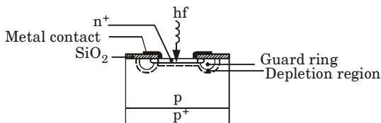
Fig. 10. Structure of a silicon avalanche photodiode with guard ring.
