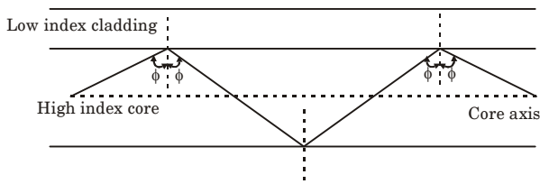
Fig. 9. The transmission of a light ray in a perfect optical fiber.
