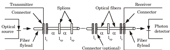
Fig. 7. Optical power loss model for a point-to-point link. The losses occur at connectors ( l_c ), at splices ( l_{sp} ), and in the fiber ( \alpha ).
