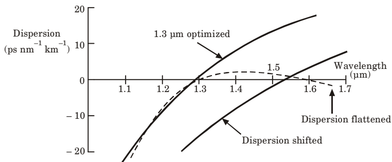
Fig. 2.17.1. Total dispersion characteristics for the various types of single-mode fiber.
