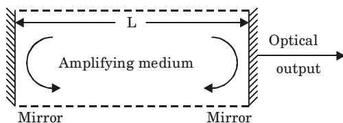
Fig. 2. The basic Laser structure incorporating plane mirrors.
