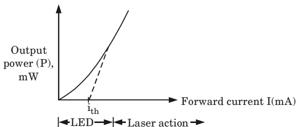
Fig. 21. Emission characteristics.
