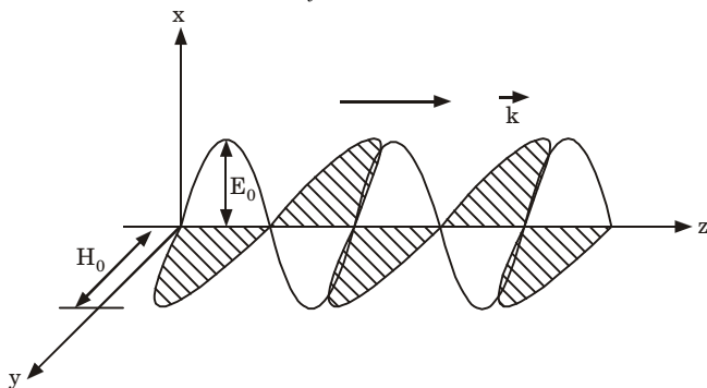
Fig. 1.12.1. A plane electromagnetic wave propagating in the + z direction.
