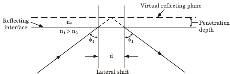
Fig. 1. The lateral displacement of a light beam on reflection at a dielectric interface (Goos-Haenchen shift).
