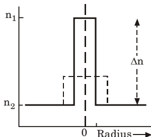
Fig. 5. Refractive index profile of a step index dispersion shifted fiber (solid) with a conventional nonshifted profile design (dashed).
