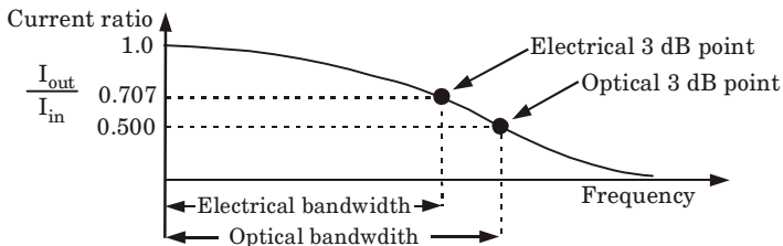
Fig. 3.6.2. The frequency response for an optical fiber system showing the electrical and optical bandwidths.
