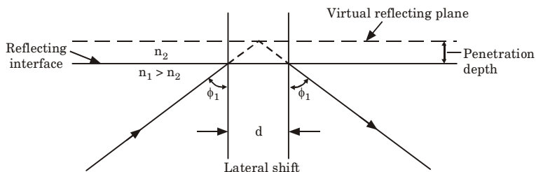
Fig. 1.17.1. The lateral displacement of a light beam on reflection at a dielectric interface (Goos-Haenchen shift).
