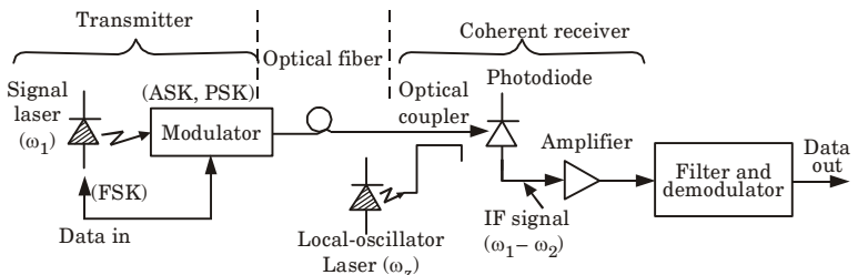
Fig. 5.7.1. Fundamental concept of coherent lightwave system. The three basic detection methods can have various modulation formats.
