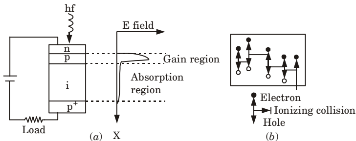
Fig. 9. (a) Avalanche photodiode showing high electric field (gain) region. (b) Carrier pair multiplication in the gain region.
