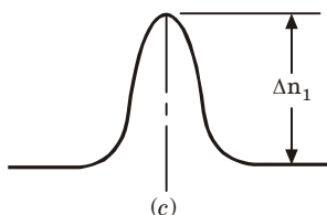
Fig. 2.18.2. Refractive index profiles for graded index dispersion shifted fibers; (a) triangular profile; (b) depressed-cladding triangular profile, (c) Gaussian profile.
