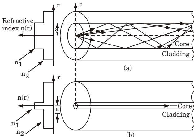
Fig. 15. The refractive index profile and transmission in step index fibers : (a) multimode step index fiber ; (b) single-mode step index fiber. \lambda = free space wavelength.
