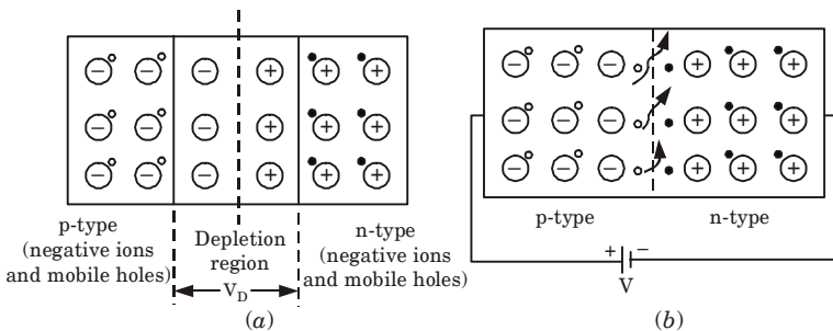
Fig. 3.1.2. Light radiation by the p - n junction of a semiconductor (a) Depletion region and Depletion voltage V_D ; (b) Light radiation as the result of electron-hole recombinations.
