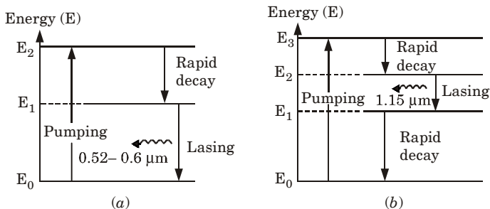
Fig. 3.13.2. Energy level diagrams showing population inversion and lasing for two non-semiconductor Lasers : (a) three level system – ruby (crystal) Laser ; (b) four level system – He-Ne (gas) Laser.
