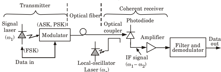
Fig. 25. Fundamental concept of coherent lightwave system. The three basic detection methods can have various modulation formats.
