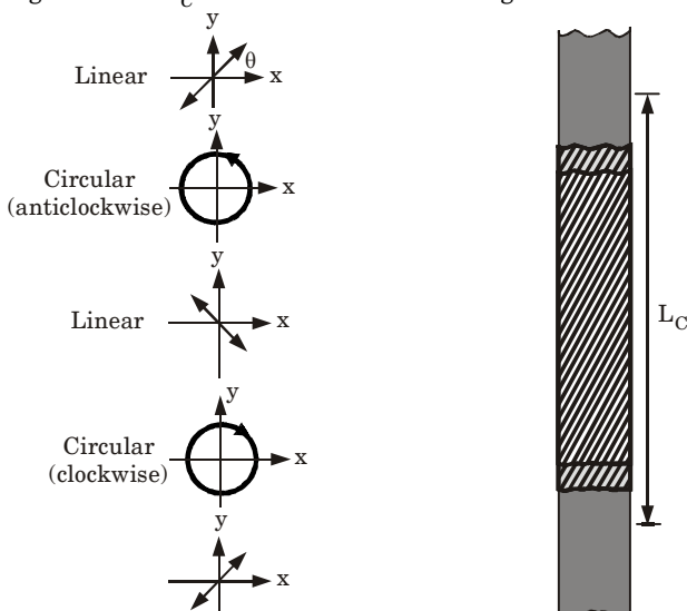
Fig. 2.20.1. An illustration of the beat length in a single mode optical fibre.
