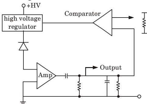
Fig. 9. Bias of an APD by peak detection and feedback to provide AGC.
