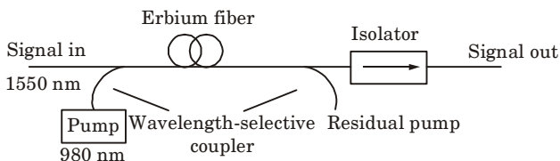
Fig. 7. An erbium-doped fiber amplifier.
