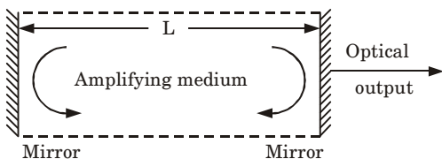
Fig. 3.17.1. The basic Laser structure incorporating plane mirrors.
