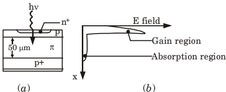
Fig. 4.13.1. (a) Structure of a silicon RAPD. (b) The field distribution in the RAPD showing the gain region across the p-n^+ junction.
