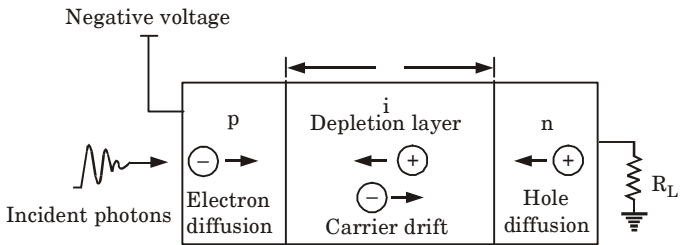
Fig. 4.15.1. Reverse biased PIN diode.
