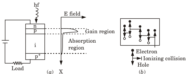
Fig. 10. Avalanche photodiode showing high electric field (gain) region. (b) Carrier pair multiplication in the gain region.
