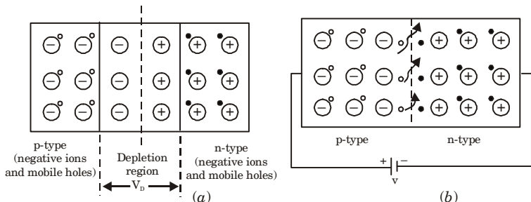
Fig. 6. Light radiation by the p-n junction of a semiconductor
